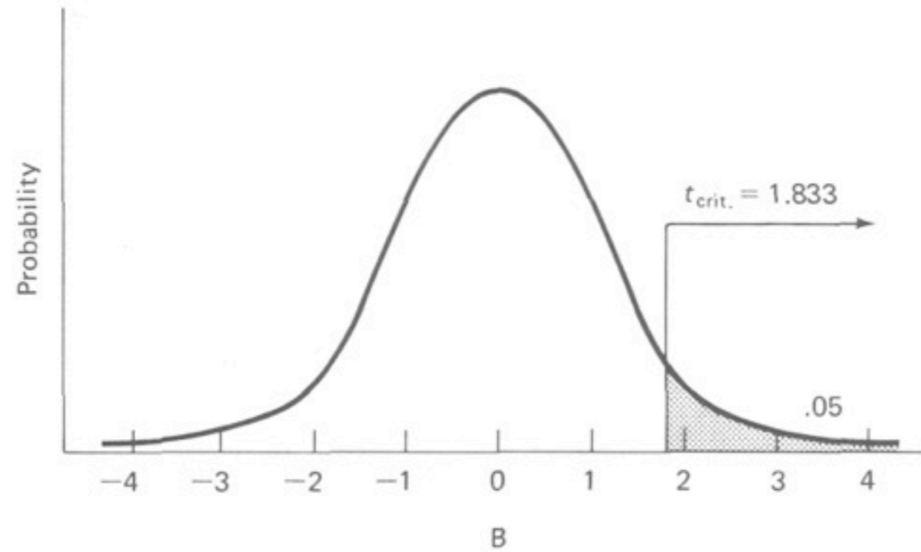
Fig. 16-1 Two-tailed (A) and one-tailed (B) rejection regions for a t distribution with 9 degrees of freedom, where the level of significance ( \alpha ) equals .05.
